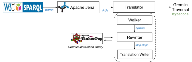
Figure 4. The sparql-gremlin query translation pipeline.
