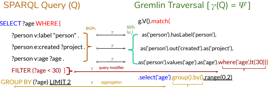
Figure 3. Illustration of a transformation from a SPARQL query ( Q ) to its Gremlin counterpart ( \Psi ).
